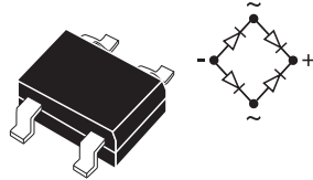
SMDIP CASE
